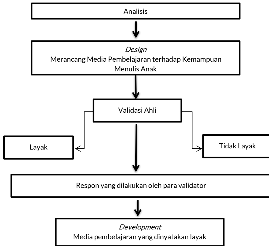
Gambar 1. Prosedur penelitian
